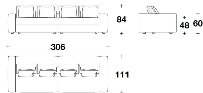
ORT (D4) DIVANO 4 POSTI IN 2 ELEMENTI / 4 SEATER SOFA IN 2 ELEMENTS 306x111x84H. - H.A.60 - H.S.48 cm 120 1/3x43 2/3x33H. - H.A.23 2/3 - H.S.19 "
