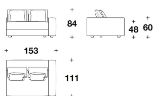
ORT (E2D) - ORT (E2S) ELEMENTO 2 POSTI CON BRACCIOLO DX O SX / 2 SEATER ELEMENT WITH RIGHT OR LEFT ARMREST 153x111x84H. - H.A.60 - H.S.48 cm 60 1/3x43 2/3x33H. - H.A.23 2/3 - H.S.19 "
